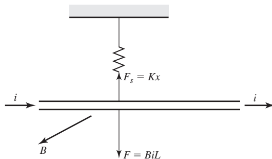
Figure 4.2 The primitive ammeter.
