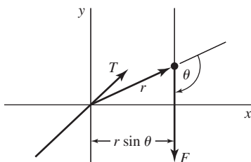
Figure 10.1 Vector representation for torque.
