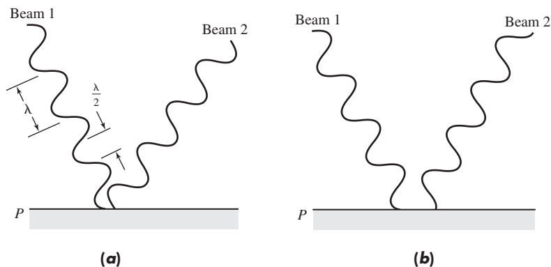
Figure 5.4 Interference principle. (a) Beams in phase; (b) beams out of phase.
