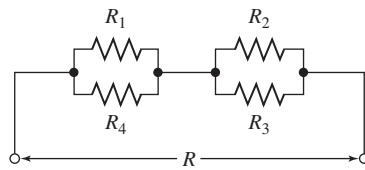
Figure 4.26 Equivalent circuit of bridge as presented to the galvanometer.
