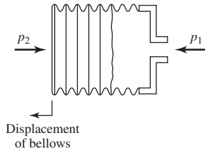
Figure 6.12 Schematic of a bellows pressure gage.
