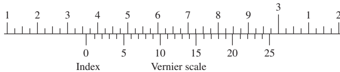
Figure 5.2 Expanded view of vernier scale.
