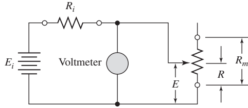
Figure 4.20 Voltage-sensitive input circuit. Change in resistance R is indicated through change in voltage indication.
