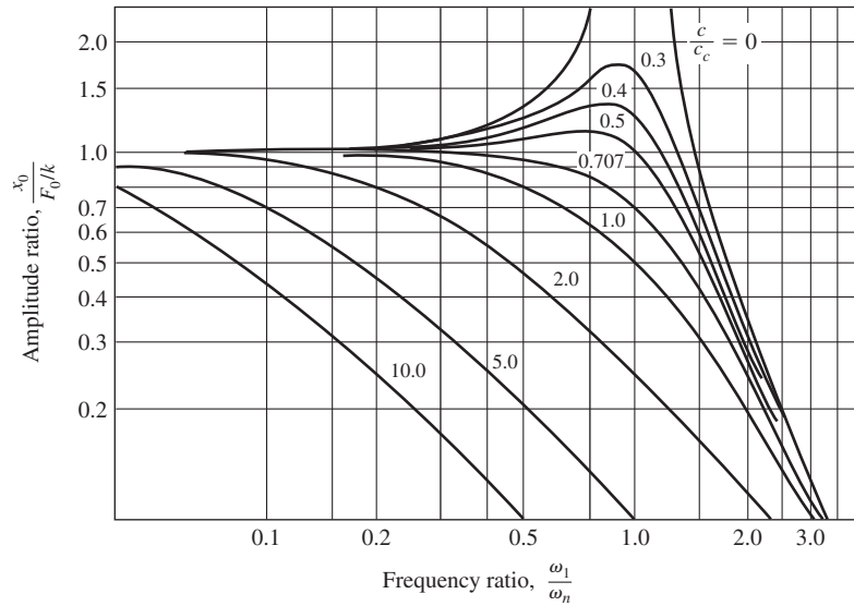
Figure 2.6 Frequency response of the system in Fig. 2.5.
