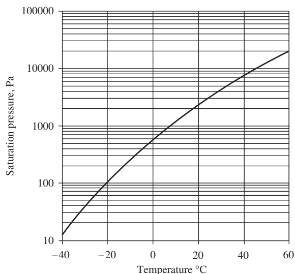
Figure 9.20 Saturation pressure for water vapor.
