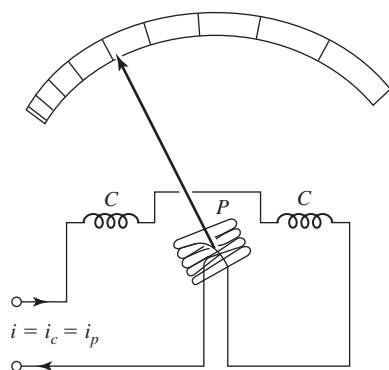
Figure 4.13 Electrodynamicometer movement used as an ammeter.
