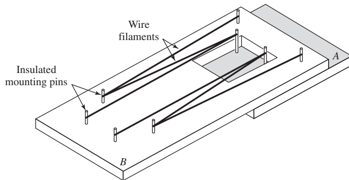
Figure 10.15 Schematic of unbonded resistance strain gage.
