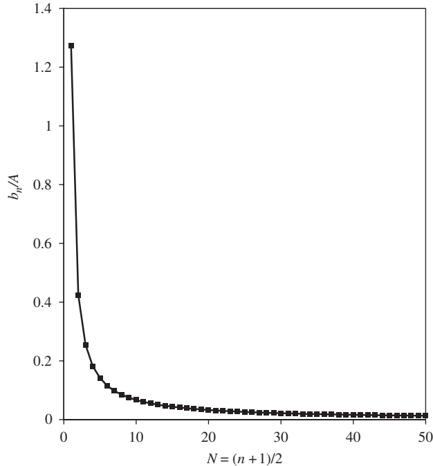
Figure 2.17 Fourier coefficients for square wave.
