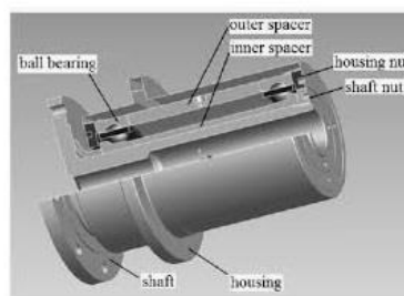
Bearing unit assembly Being a critical ... researchgate.net
