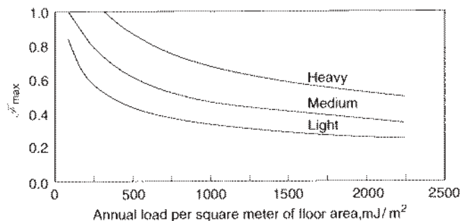
Figure 22.5.3 The \mathcal{F}_{\max} as function of annual load per square meter of floor area and building construction for an allowable temperature swing of 7^{\circ}\text{C} . From Evans and Klein (1984a).
