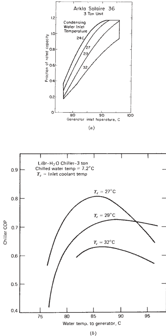
Figure 15.2.4 Manufacturer's data for 3-ton Arkla LiBr-H 2 O water chiller showing (a) capacity as a function of water inlet temperatures to generator and condenser at chilled water outlet temperature of 7.2 °C, and (b) COP as a function of water inlet temperatures to generator and condenser. From Blinn (1979).
