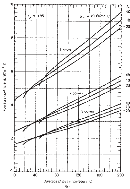
Figure 6.4.4 Top loss coefficient for slope of 45^\circ and a plate spacing of 25 mm.
