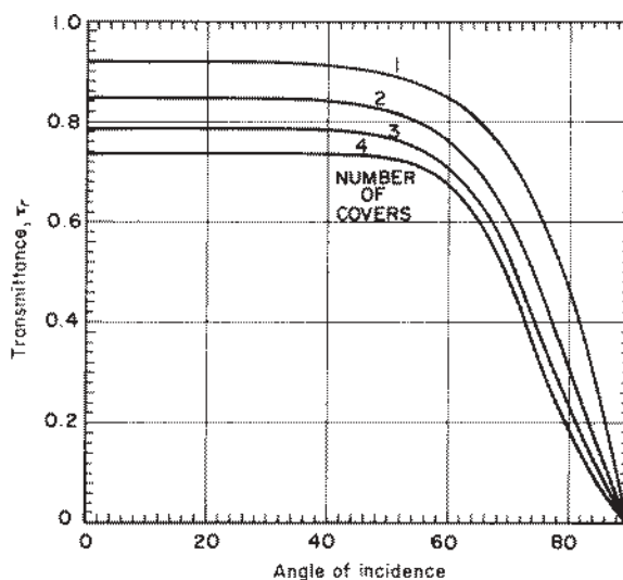
Figure 5.1.3 Transmittance of 1, 2, 3, and 4 nonabsorbing covers having an index of refraction of 1.526.
