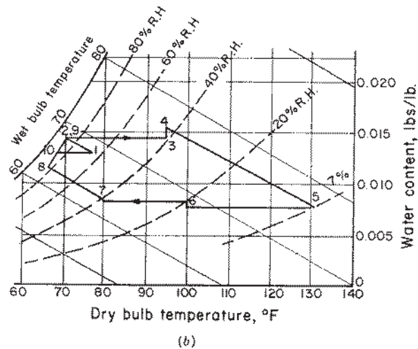
Figure 15.7.2 (a) Schematic of open-cycle solar air conditioning system using a rotary desiccant bed and heat exchangers. (b) The cycle on a psychrometric chart. From Dunkle (1965).
