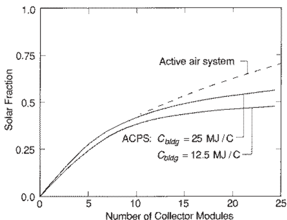
Figure 14.8.2 Solar contributions in Springfield, IL, of ACPS systems with building thermal capacitances of 25 and 12.5 \text{ MJ}/^\circ\text{C} and an active air system; (UA)_h = 200 \text{ W}/^\circ\text{C} .
