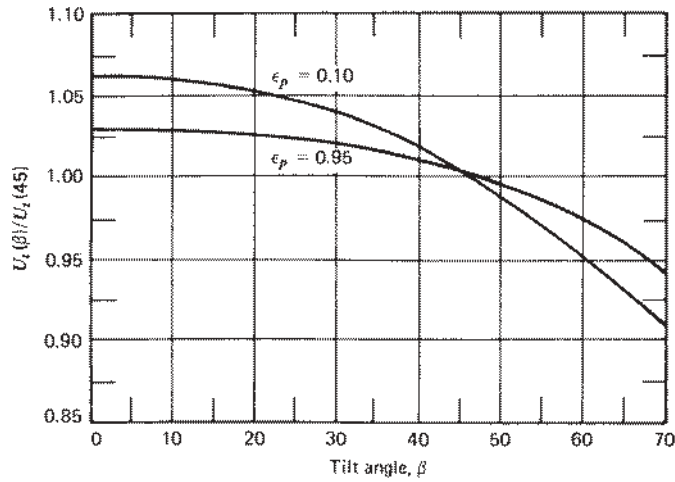
Figure 6.4.6 Dependence of top loss coefficient on slope.
