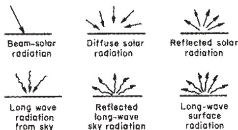
Figure 2.1.1 The radiant energy fluxes of importance in solar thermal processes. Short-wave solar radiation is shown by \rightarrow . Longwave radiation is shown by \curvearrowright .
