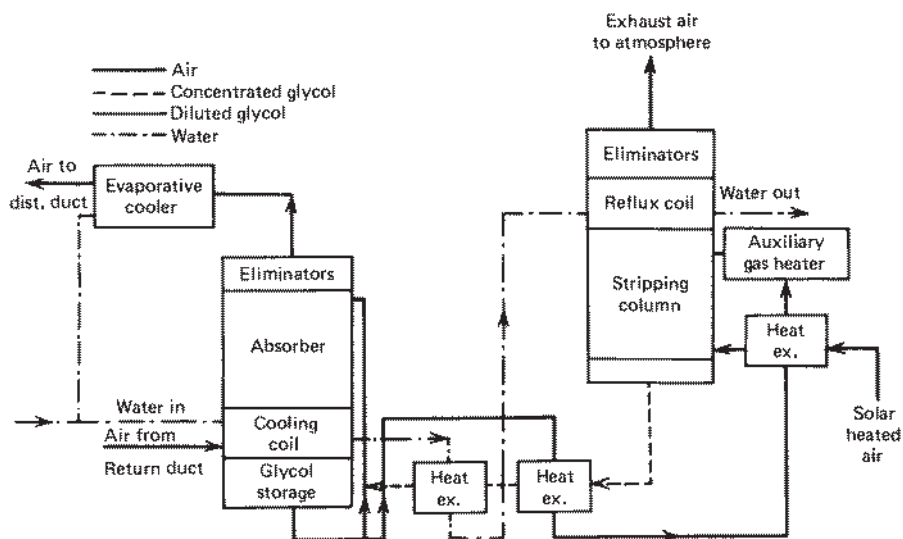
Figure 15.7.1 Schematic of a triethylene glycol open-cycle air conditioning system. From Löf (1955).
