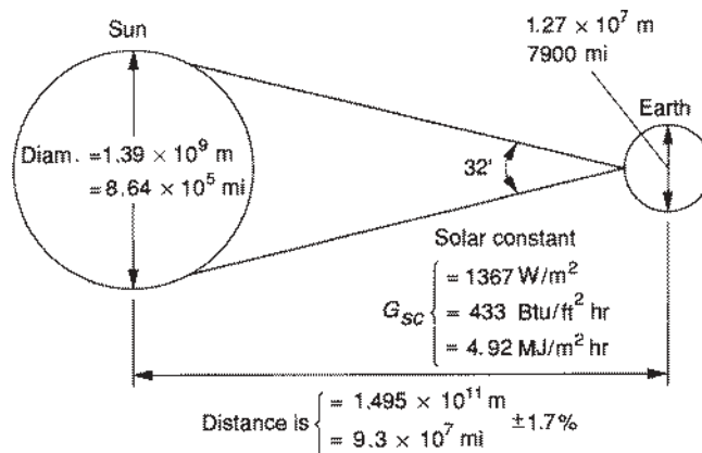
Figure 1.2.1 Sun-earth relationships.
