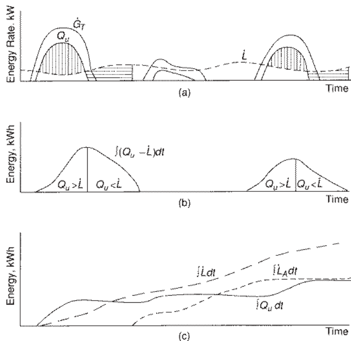
Figure 8.1.1 A solar energy process with storage. (a) Incident solar energy \dot{G}_T , collector useful gain \dot{Q}_u , and loads \dot{L} as functions of time for a three-day period. Vertical shaded areas show times of excess energy to be added to storage. Horizontal shaded areas show energy withdrawn from storage to meet loads. Dotted areas show energy supplied to load from collector during collector operation. (b) Energy added to or removed from storage, taking time t = 0 as a base. (c) Integrated values of the useful gain from collector, the load, and the auxiliary energy for the same three-day period. In this example solar energy collected is slightly more than half the integrated load.
