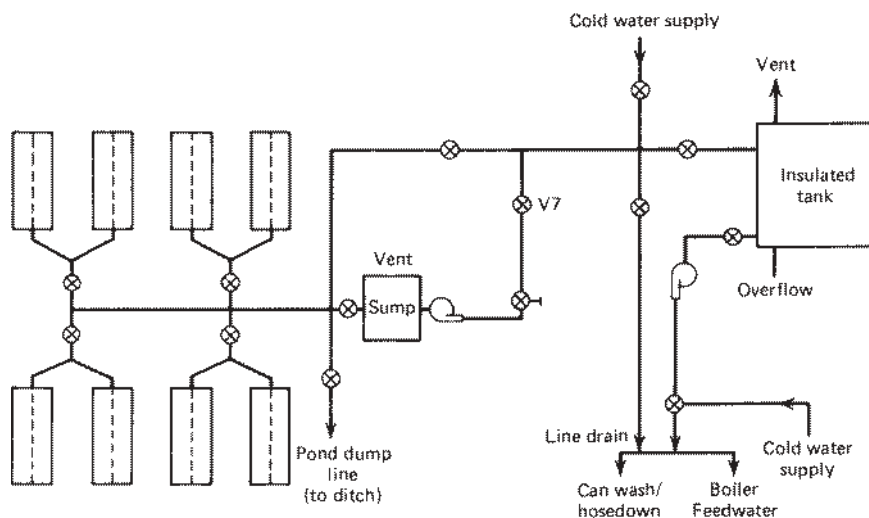
Figure 16.8.2 Schematic intermittent shallow-pond solar water heating system for a poultry processing plant. Adapted from Guinn and Hall (1977).
