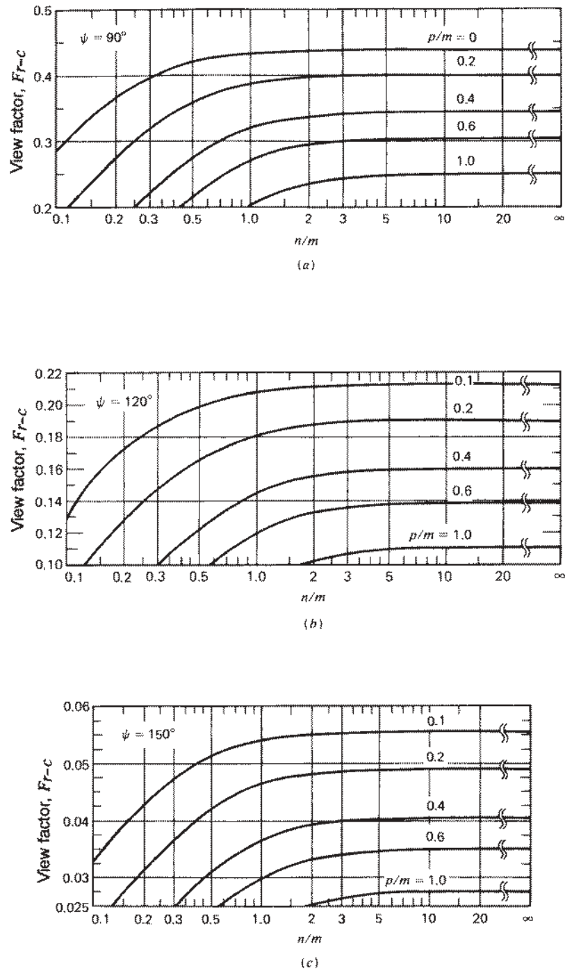
Figure 2.17.2 View factor F_{r-c} as a function of the relative dimensions of the collecting and reflecting surfaces. Adapted from Hamilton and Morgan (1952).
