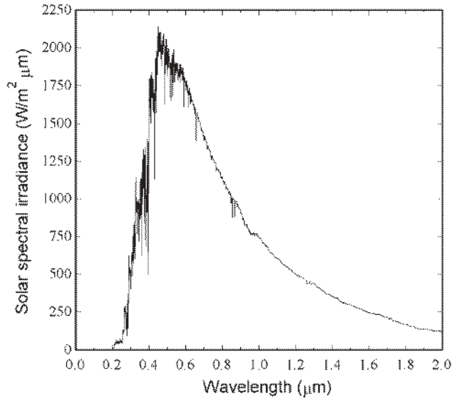
Figure 1.3.1 The WRC standard spectral irradiance curve at mean earth-sun distance.
