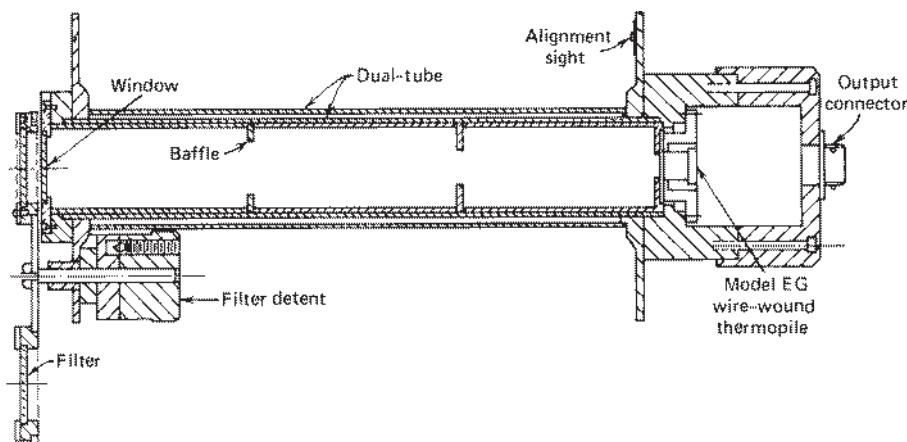
Figure 2.2.2 Cross section of the Eppley NIP. Courtesy of The Eppley Laboratory.
