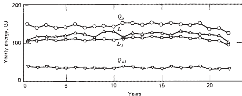
Figure 13.8.2 Year-to-year variation of performance of the 50-m 2 system with a storage capacity of 5500 liters/m 2 . From Braun (1980).
