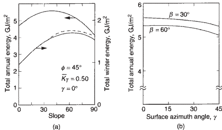
Figure 2.21.2 (a) Variation of total annual energy and total winter (December to March) energy as a function of surface slope for a latitude of 45^\circ , \overline{K}_T of 0.50, and surface azimuth angle of 0^\circ . Ground reflectance is 0.20 except for the dashed curve where it is taken as 0.60 for January and February. (b) Variation of total annual energy with surface azimuth angle for slopes of 30^\circ and 60^\circ , latitude of 45^\circ , \overline{K}_T of 0.50, and ground reflectance of 0.20.
