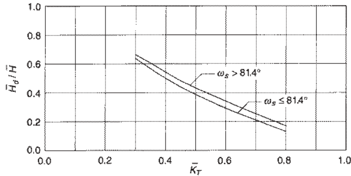
Figure 2.12.2 Suggested correlation of \overline{H_d}/\overline{H} versus \overline{K_T} and \omega_s . Adapted from Erbs et al. (1982).
