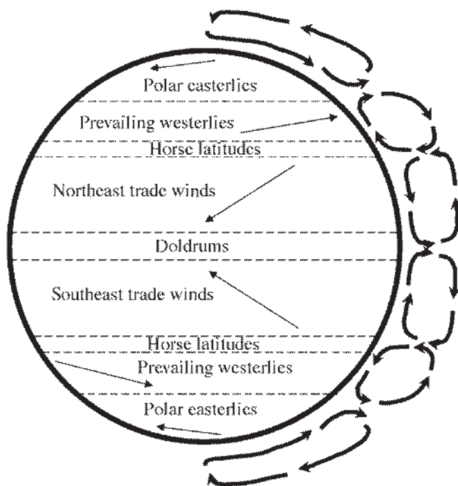
Figure 24.2.1 Planetary wind patterns.
