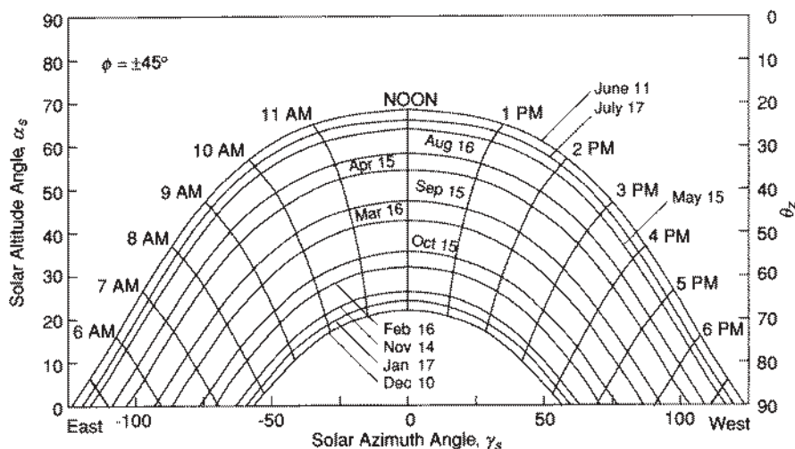
Figure 1.9.1 Solar position plot for \pm 45^\circ latitude. Solar altitude angle and solar azimuth angle are functions of declination and hour angle, indicated on the plots by dates and times. The dates shown are for northern hemisphere; for southern hemisphere use the corresponding dates as indicated in Figure 1.8.2.
