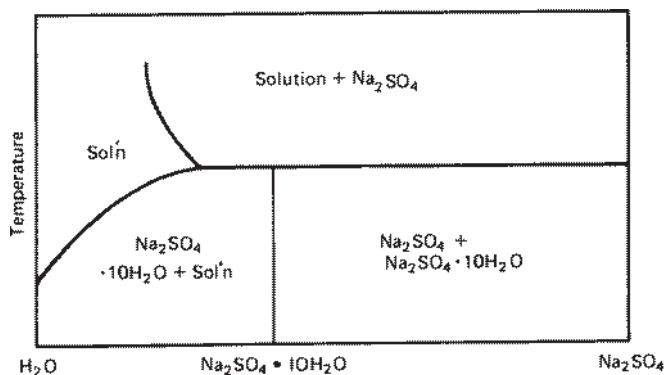
Figure 8.8.1 Phase diagram for sodium sulfate decahydrate, with incongruent melting point.
