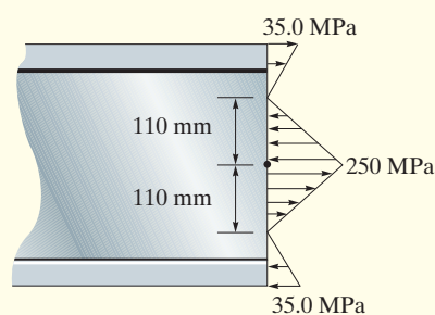
Residual stress distribution
