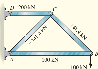
Real forces
