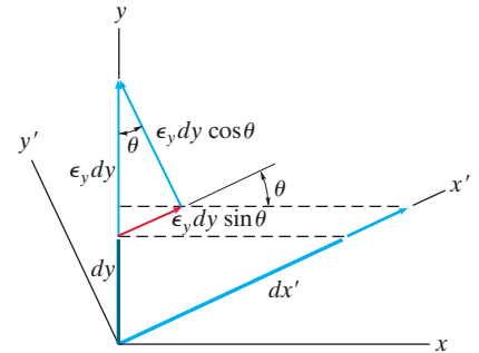
Normal strain \epsilon_y
