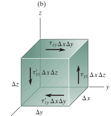
Free-body diagram
