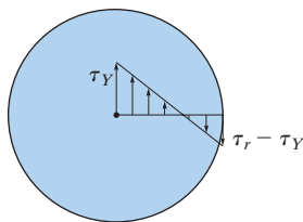
Residual shear-stress distribution in shaft (c)
