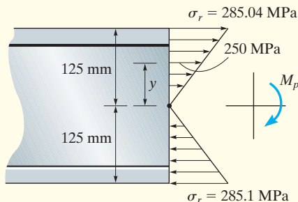
Plastic moment reversed (profile view)
