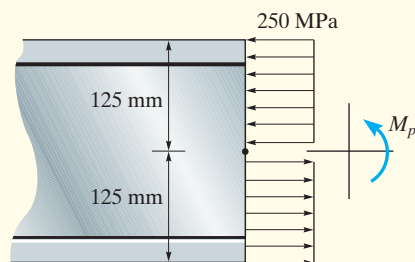
Plastic moment applied (profile view)
