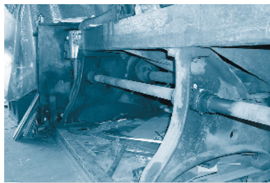
The shaft of this cutting machine is fixed at its ends and subjected to a torque at its center, allowing it to act as a torsional spring.
