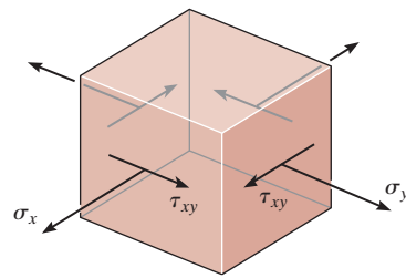
Plane stress
